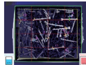
Model-less recognition
