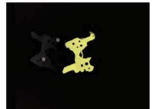
Model-matching recognition
